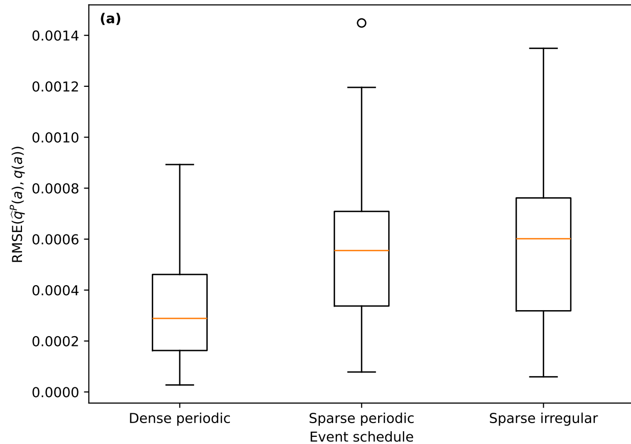
Recovery of \hat{q}^P(a)
